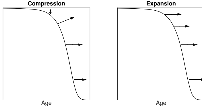
Figure 9: Different views of future survival probability: compression (lefthand graph) and expansion (righthand graph).
