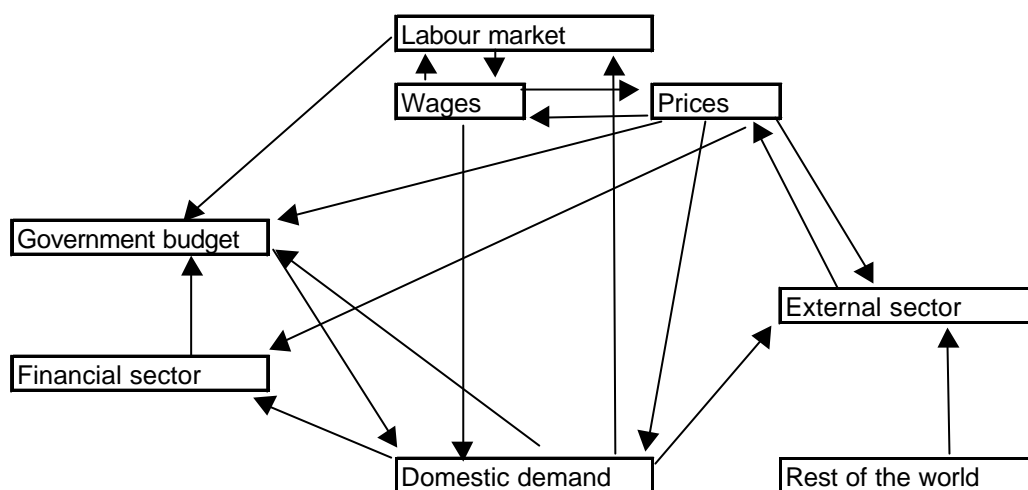
Chart 7 Model linkages
