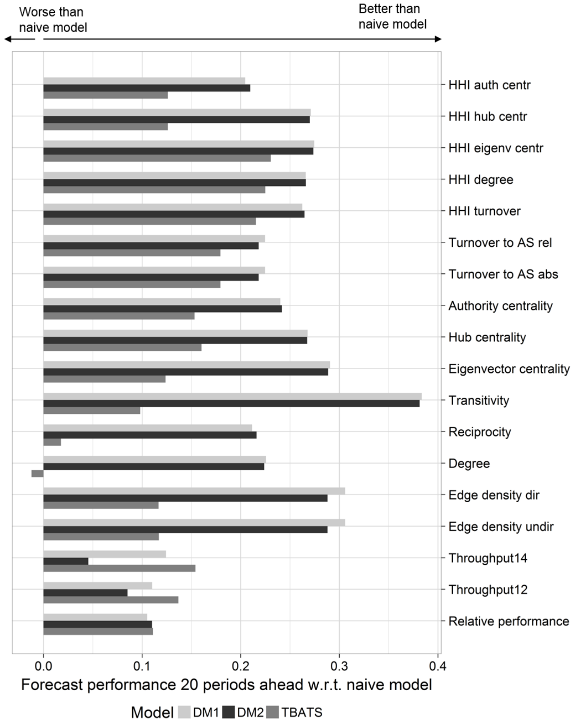
Figure 3: Out-of-sample fit of all indicators for 1.1 and 1.2 transactions with respect to the naive model.
