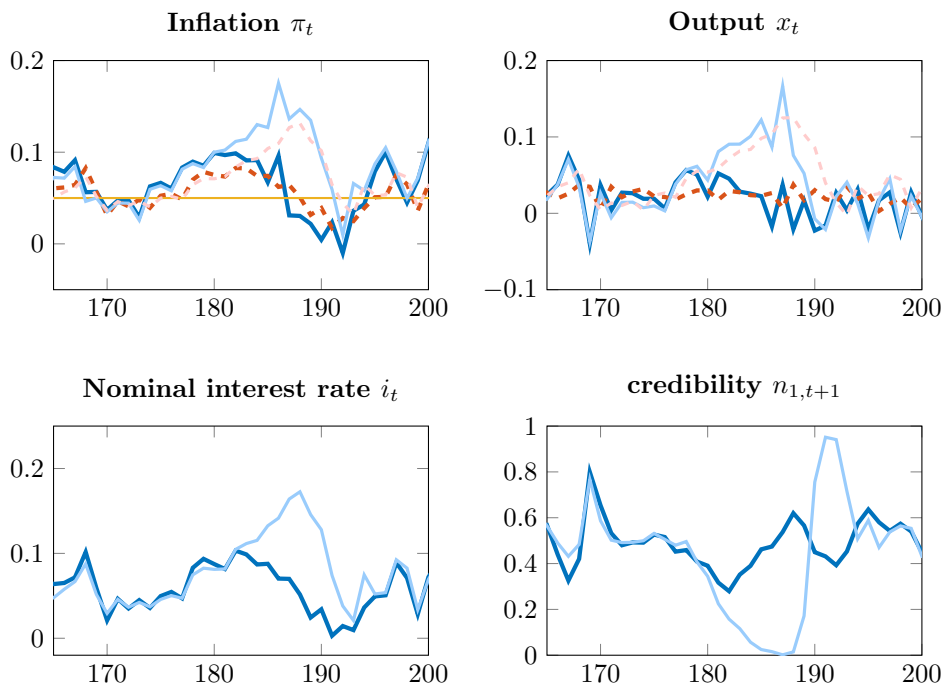
Figure 5: Constant vs. decreasing gain in the central bank’s learning algorithm
