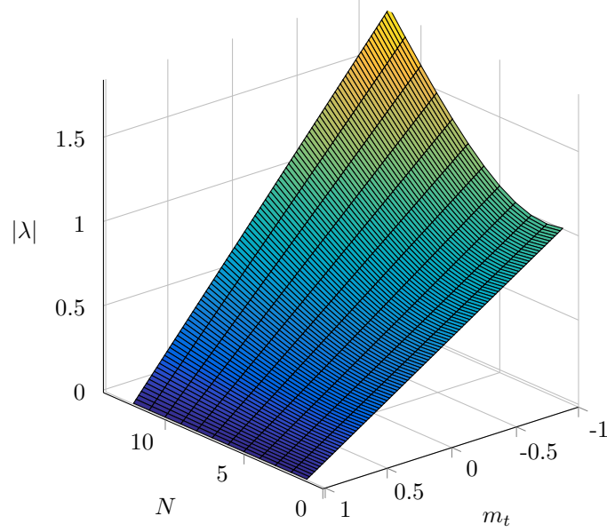
Figure 7: Absolute eigenvalue |\lambda_1| as a function of N and m_t .
