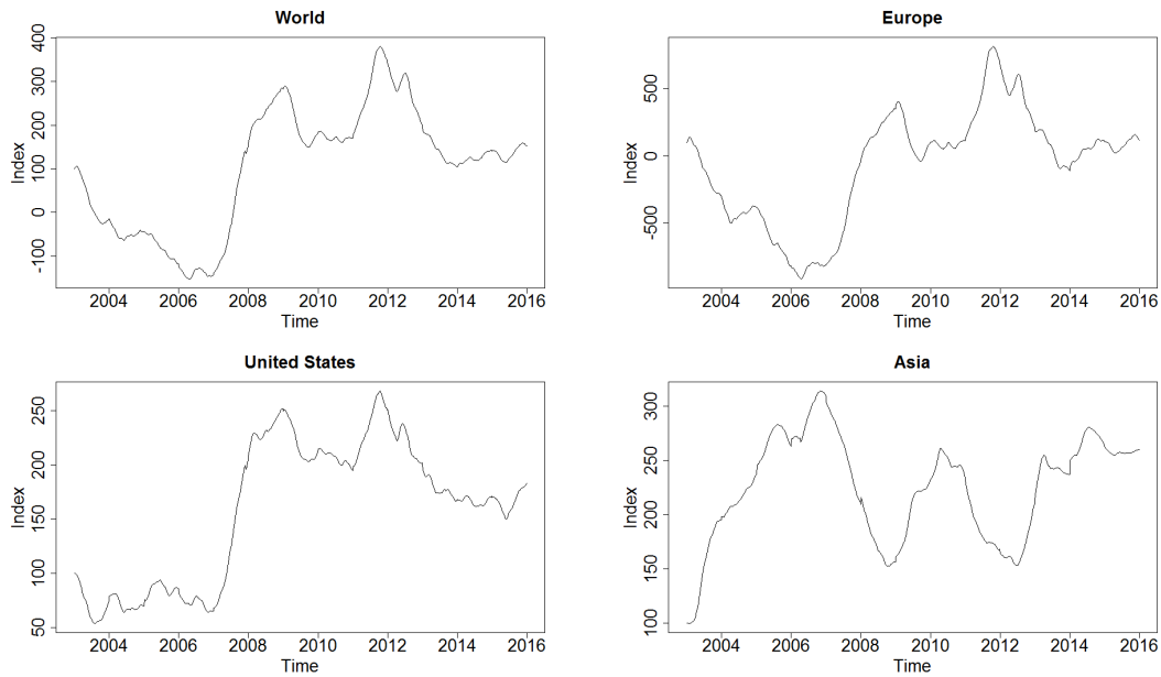
Figure 4: Historical SenSR for different regions
