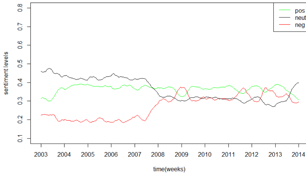
Figure 2: Example of Kalman-Filtered News Sentiment Probabilities (Company: HSBC)
