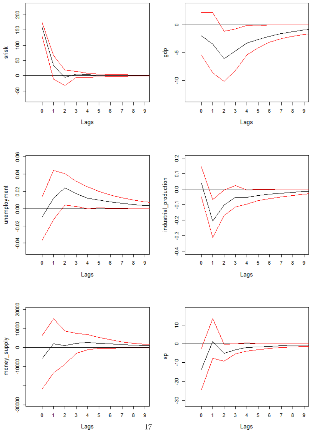
Figure 7: Impulse response function: SRISK global on US Macro Data for VAR(1)
