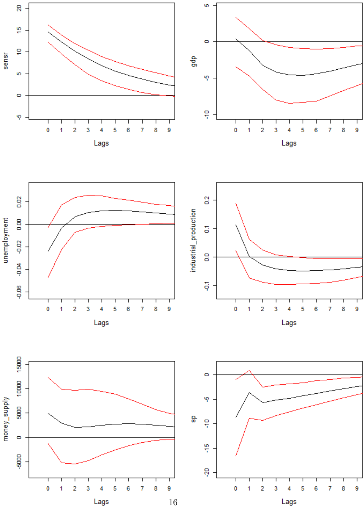
Figure 6: Impulse response function: SenSR on US Macro Data for VAR(1)
