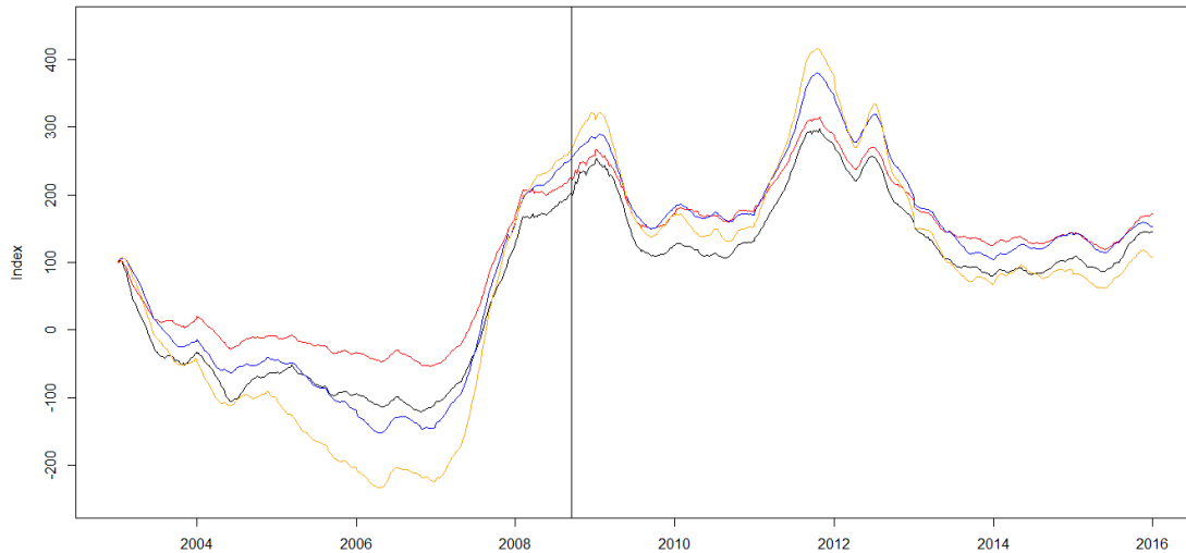
Figure 3: Historical SenSR. Black: market Value weights, blue: leverage, red: market value and leverage, orange: debt.
