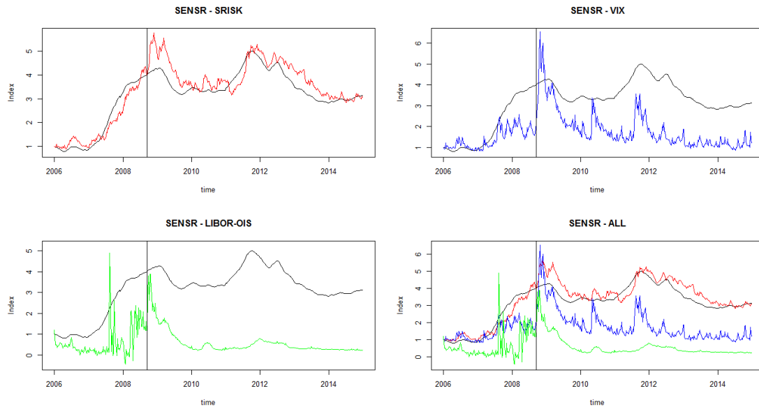
Figure 5: SenSR compared to other systemic risk indicators.
