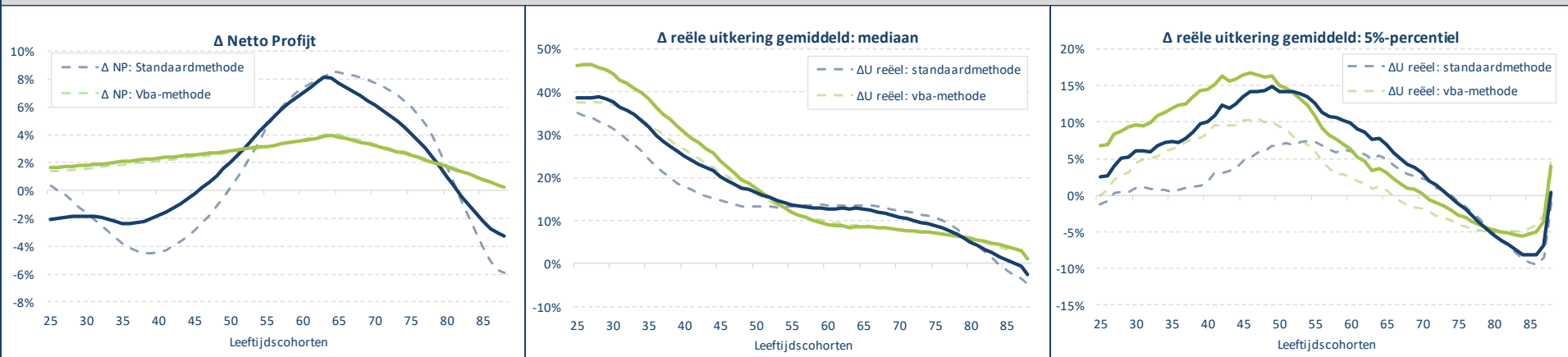
renteschok +100bps
