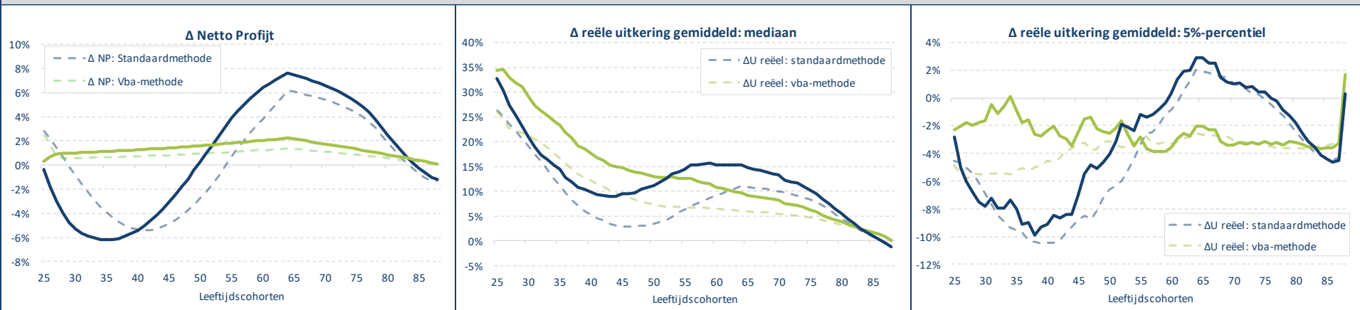
Cie19: Basis
