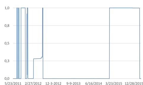
Figure 10. Regime switches safe asset market
