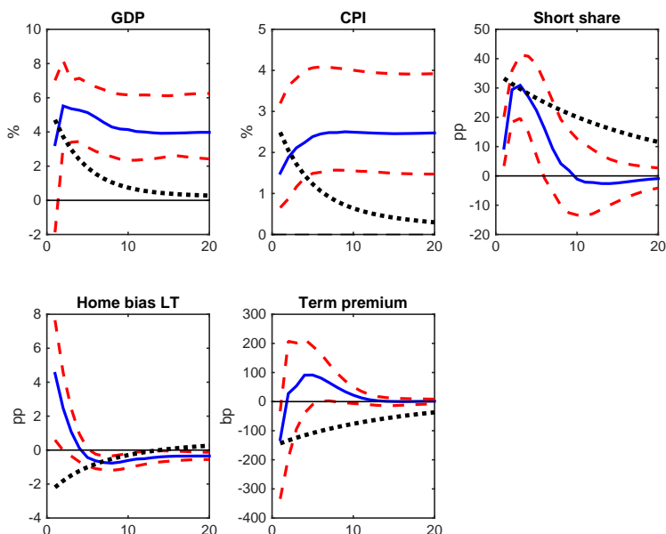
Figure 16: SVAR: QE Shock in the Core
