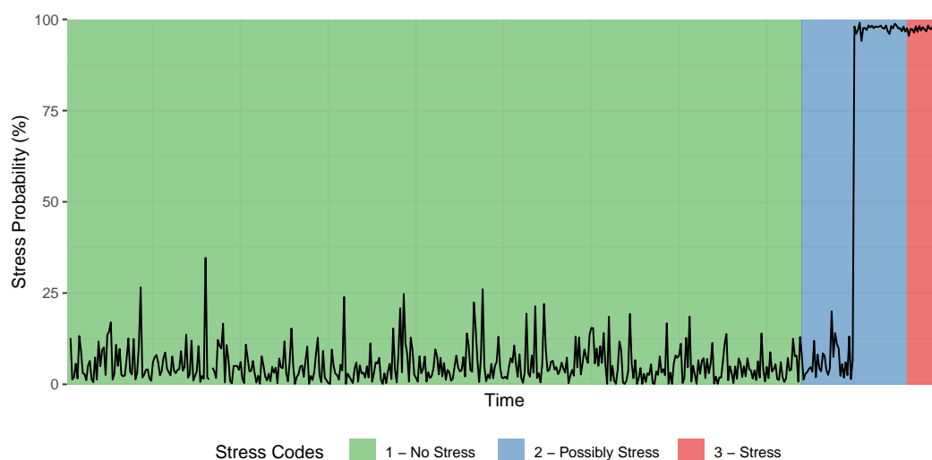
Figure 2: The out-of-sample predictions of MLP2 for bank E. The background colors highlight the stress codes that were assigned to the feature vectors of the bank by our news analysis. The classifier picks up an early-warning sign of liquidity stress in the 'Possibly Stress' period, quite some time before newspapers reported the stress in the 'Stress' period. Note that, because of confidentiality reasons, we were not allowed to include the original figure in this paper. This figure is artificially generated and closely resembles the original figure.
